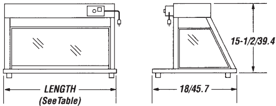
Model HFC-xx Shown
