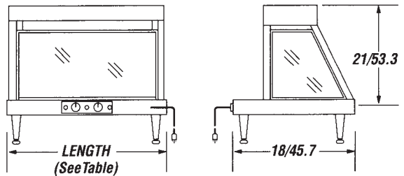
Model HFC-TS-xx Shown
